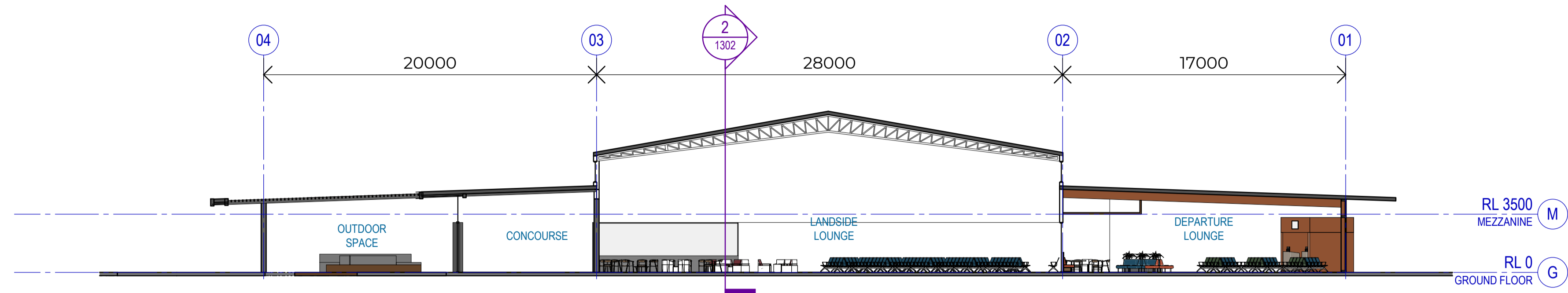
1 Section A SCALE 1:200
